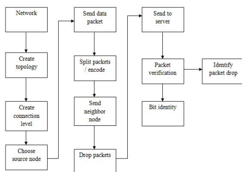
Fig2: System architecture
